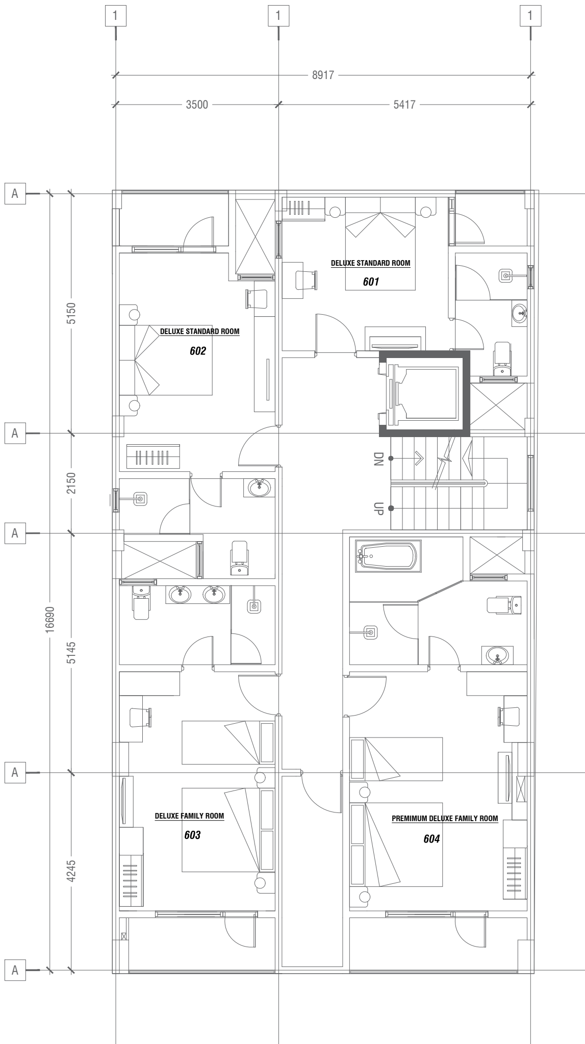
6TH FLOOR PLAN
