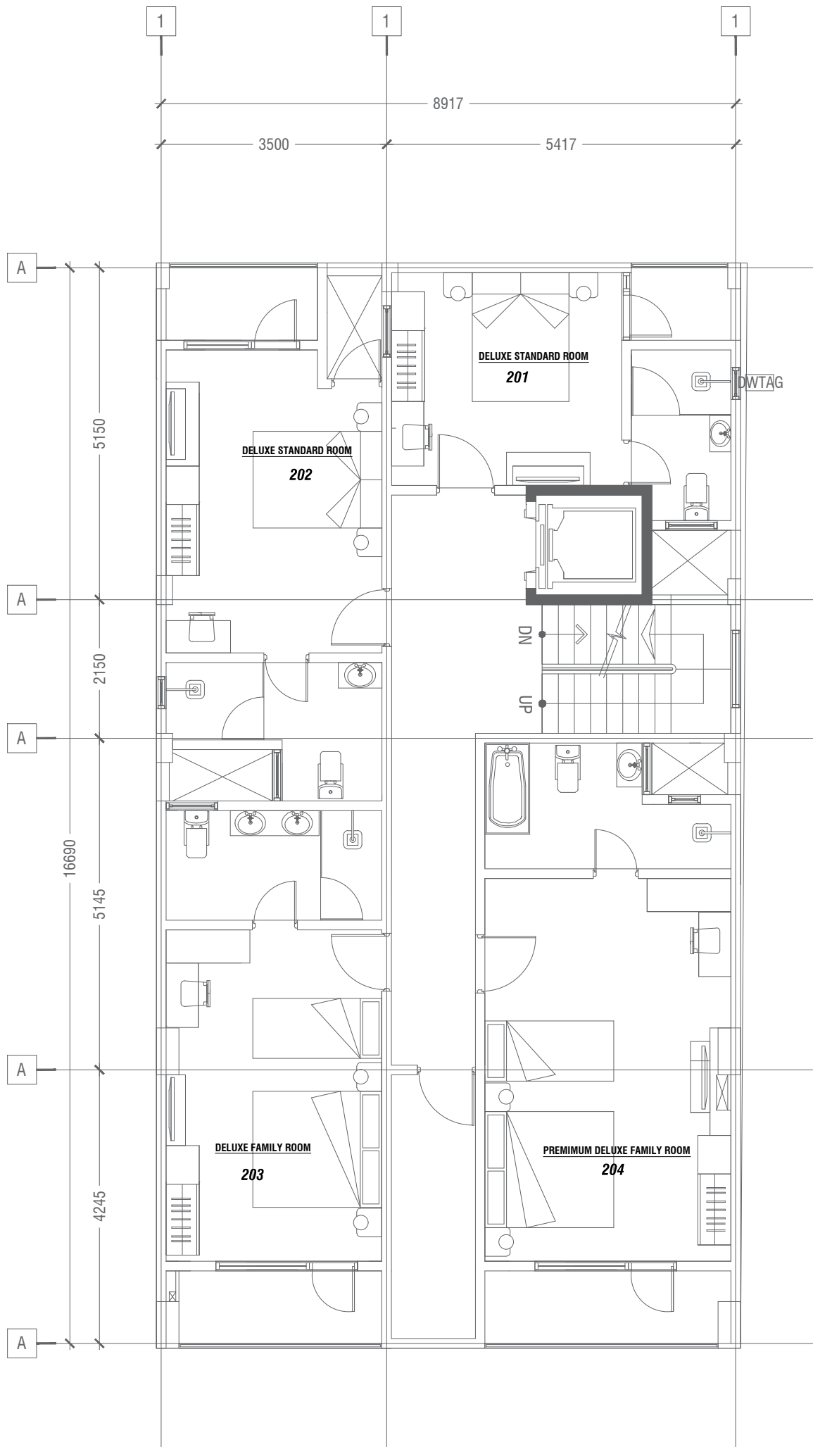
2ND FLOOR PLAN
